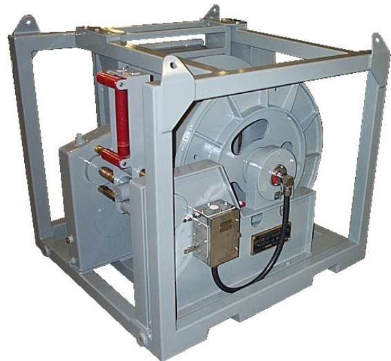
SPR-1238 showing EX slipring and junction box
